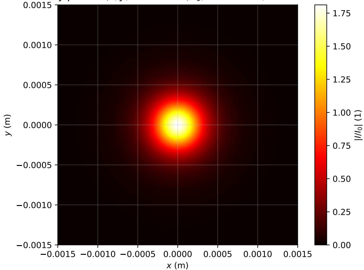
Intensity profile I(x, y, z = 1.433m)/I_0 , P_{in}=1.0P_{cr} , artificial time
